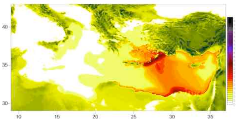
Maximum wave height distribution of the Mw=8.4 worst-case interpretation of the 1303 Eastern Mediterranean earthquake used in NEAMWave12 by KOERI (left) and KOERI's Operations Room during the Exercise (right)
