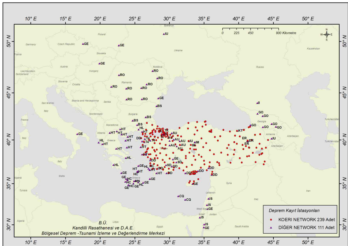
Distributions of national and regional seismic stations around Turkey available with real-time data.
