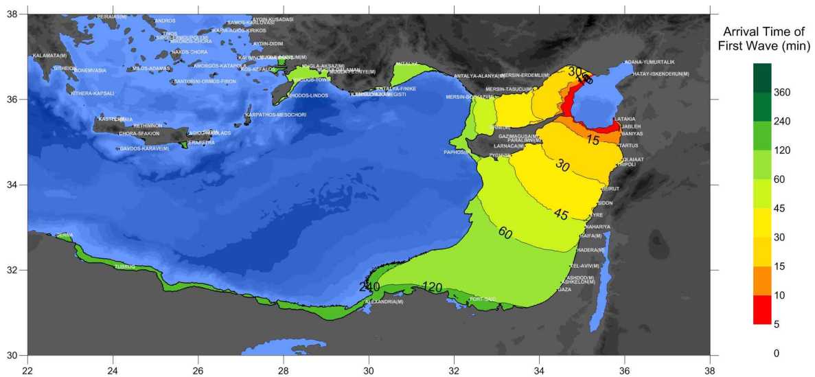
Arrival times of first wave in the KOERI M7.4 Samandag scenario during NEAMWave17
